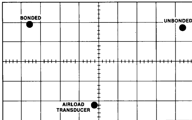
FIGURE 1 A display of the transducer impedance from the Bondascope 2100.
