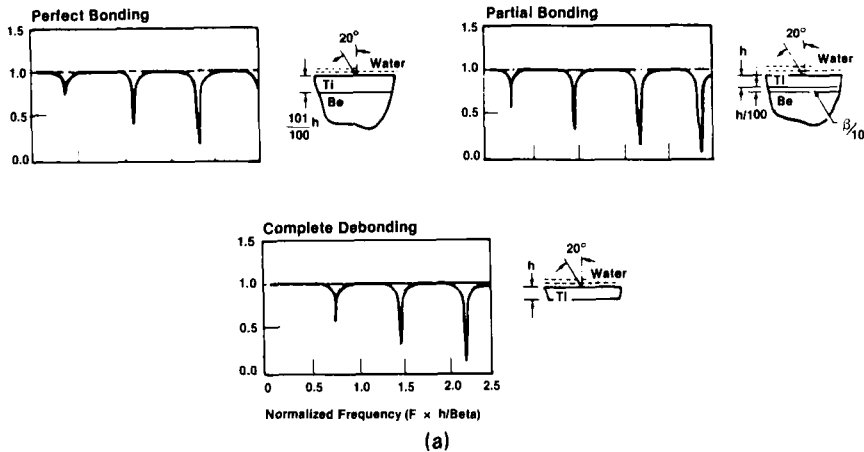
DISPERSION CURVES TI (0.04 mm) /INTERFACE (0.0004 mm) /Be (HALF SPACE)
