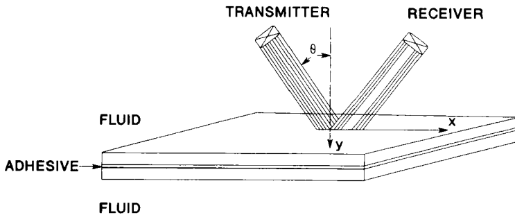
FIGURE 11 Schematic diagram of the leaky Lamb Wave (LLW) field.
