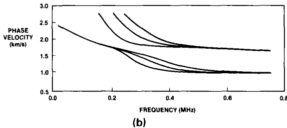
FIGURE 15 The influence of bond properties on the phase velocity of Lamb waves. The single-layered medium consists of a layer of Titanium bonded to a Beryllium substrate, with perfect bonding, with a thin low-velocity interfacial layer and with complete debonding at the interface. The reflection amplitude spectra for the three cases are shown in (a), and the corresponding dispersion curves for the first two modes in (b). \beta is the shear wave speed in Titanium.
